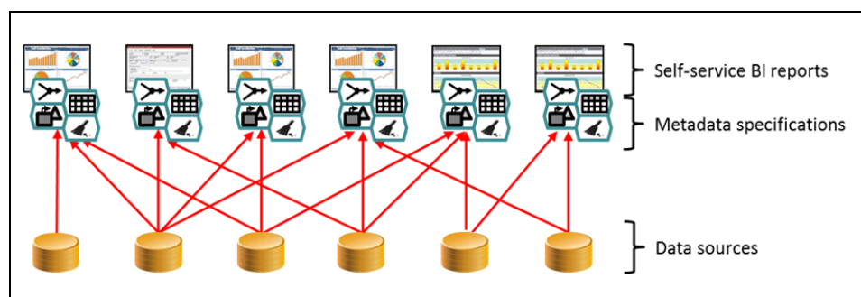
Figure 4 Self-service BI can lead to proliferation of metadata specifications.
