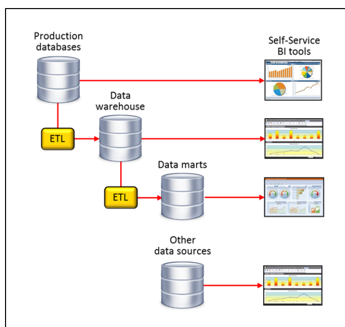
Figure 5 Self-service BI tools can directly access data sources, such as a production system, a data warehouse, or some other source.
