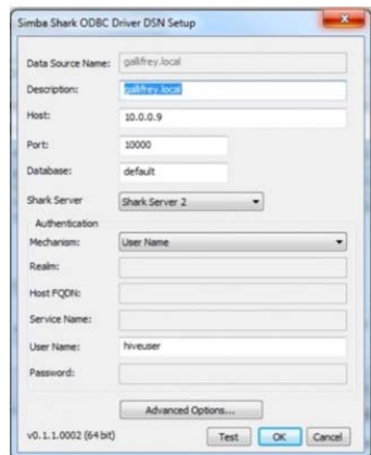
Figure 1 Connection specifications are usually entered by filling in the fields.
