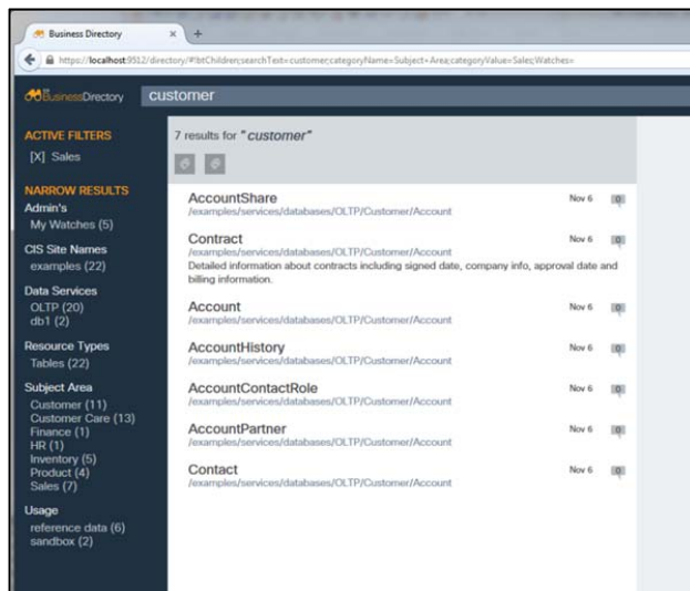
Figure 12 Searching for business objects with CBD.
